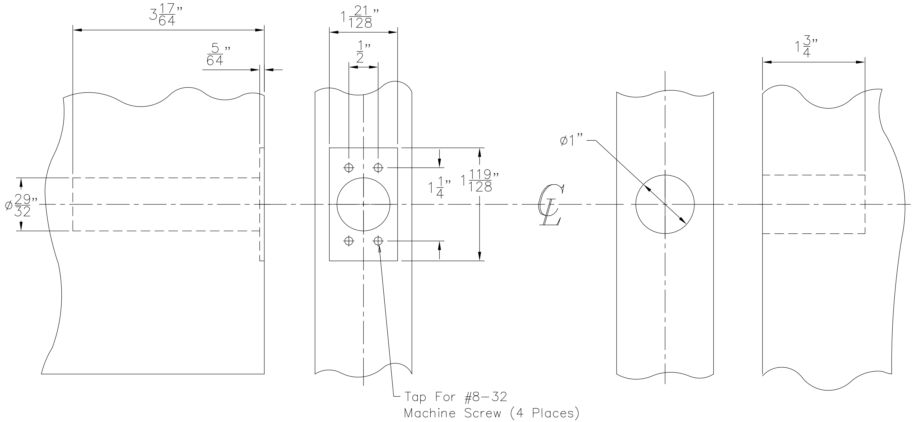
SIDE VIEW
